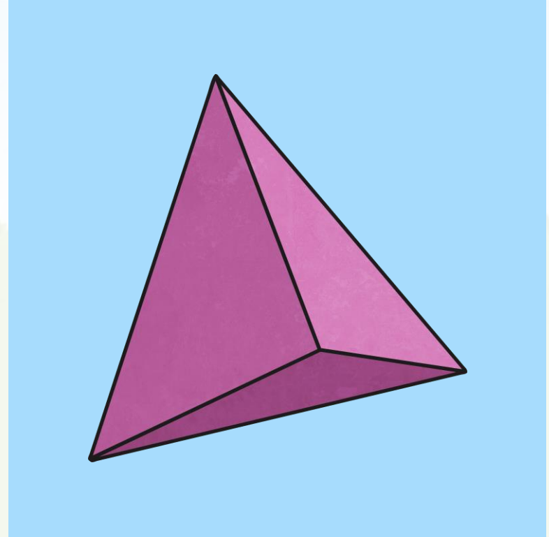
Triangular Pyramid
