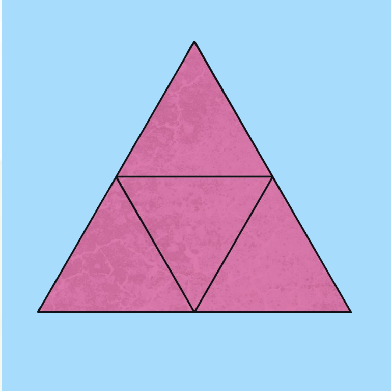
Triangular Pyramid
